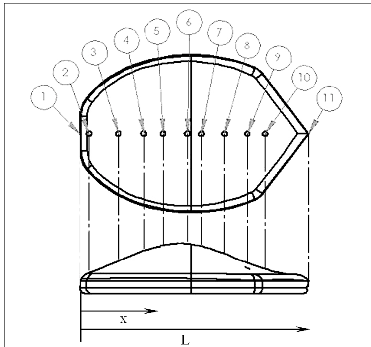
Figure 3: Pressure-tapping numbering
