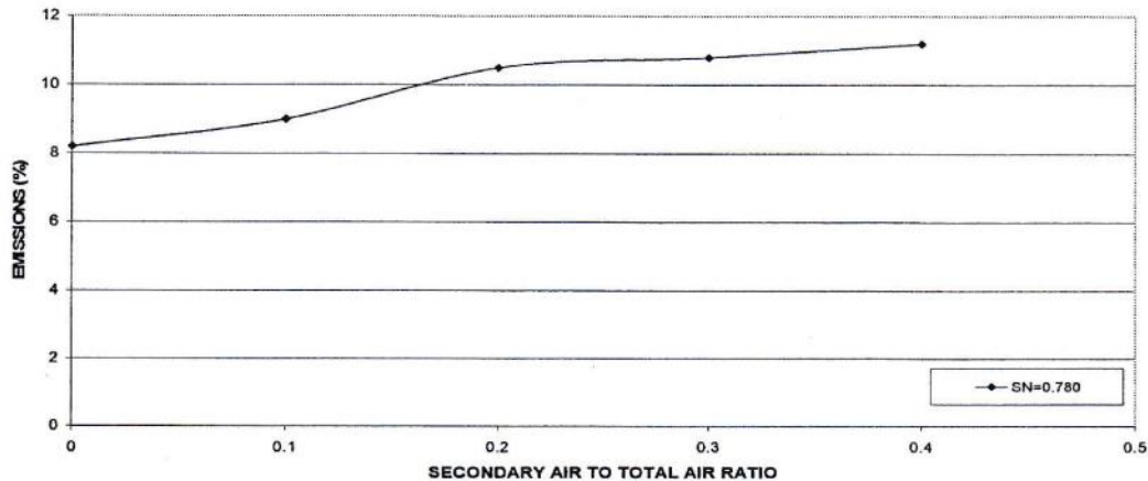
Figure 5: CO 2 vs Air ratio
