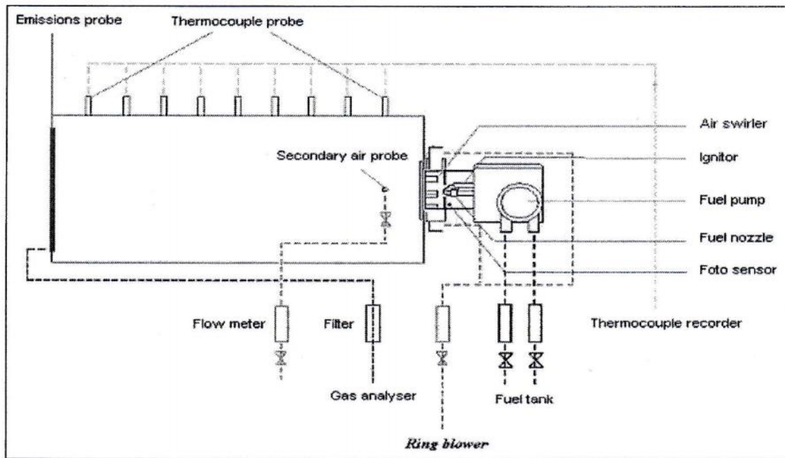
Figure 2: Schematics diagram of the liquid fuel burner
