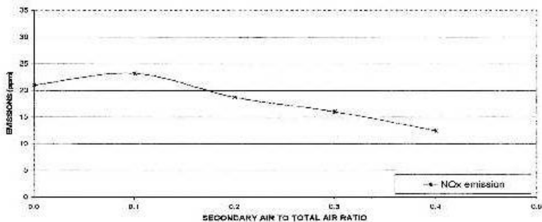
Figure 3: NO x vs air ratio
