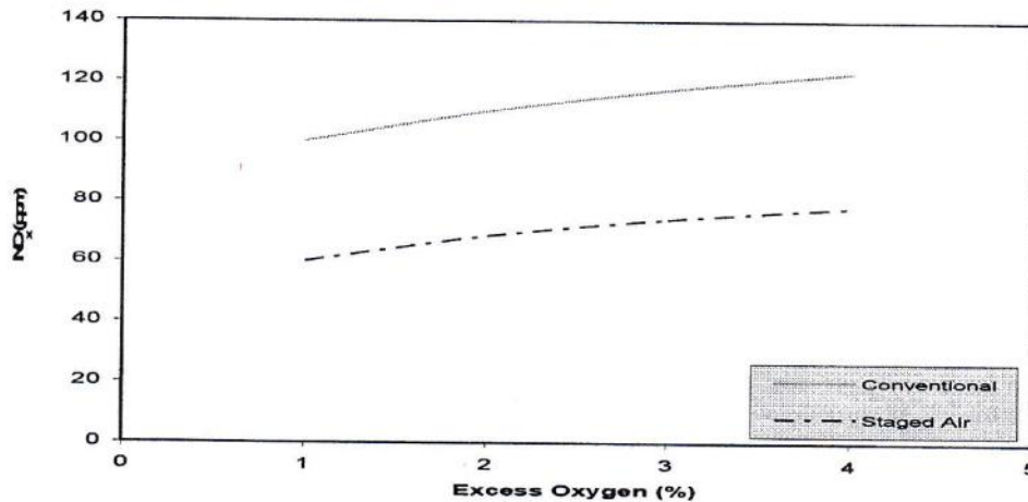
Figure 1: Comparison of conventional burner and burner with staging operation [5]
