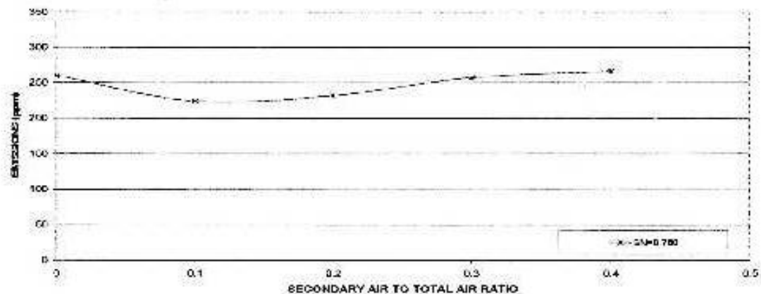
Figure 4: CO vs air ratio
