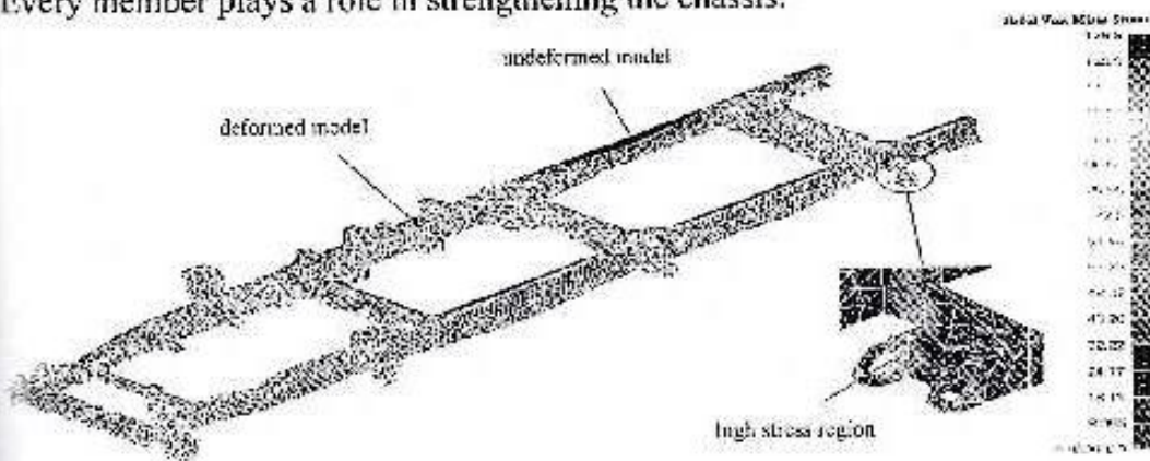
Figure 5: Stress contour and deformation pattern of the chassis under truck components loading
