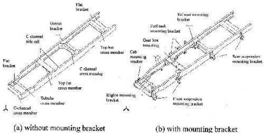
Figure 1: Truck chassis
