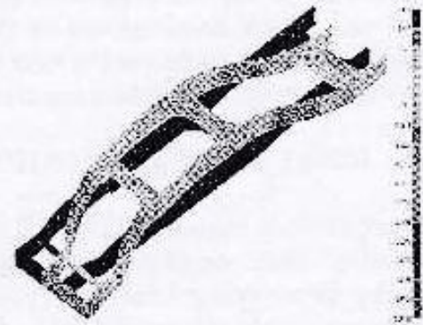
Mode 2: 34.23 Hz Global: 2 nodal points lateral bending
