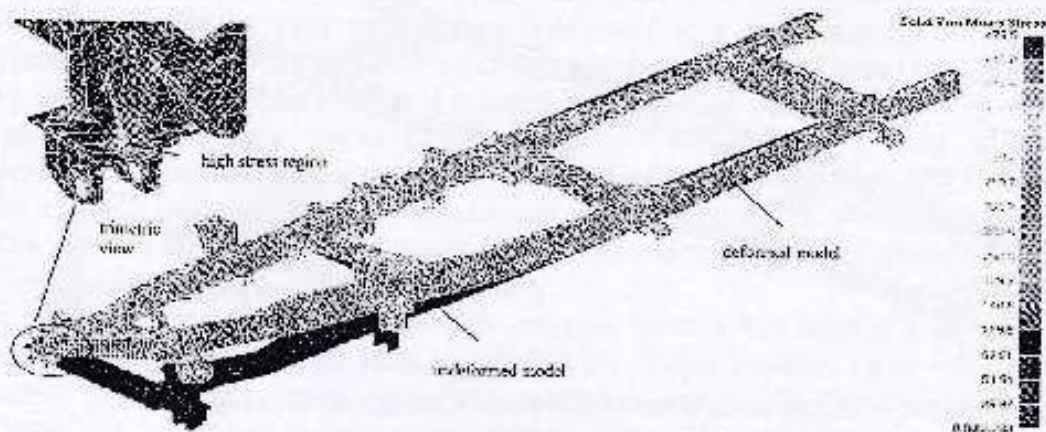
Figure 7: Stress contour and deformation pattern of the chassis under asymmetrical loading
