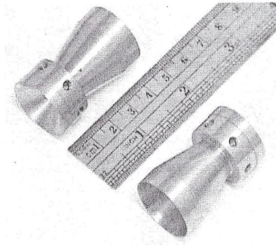
Figure 6 Convergent-divergent nozzle for rocket motor
