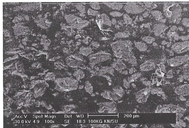
Figure 1 Propellant grain
