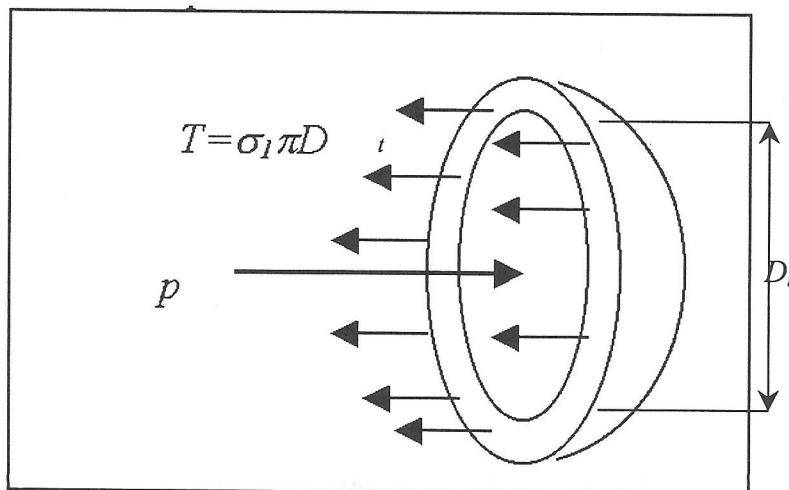
Figure 4 Free-body diagram of a portion of the cylinder cross-section
