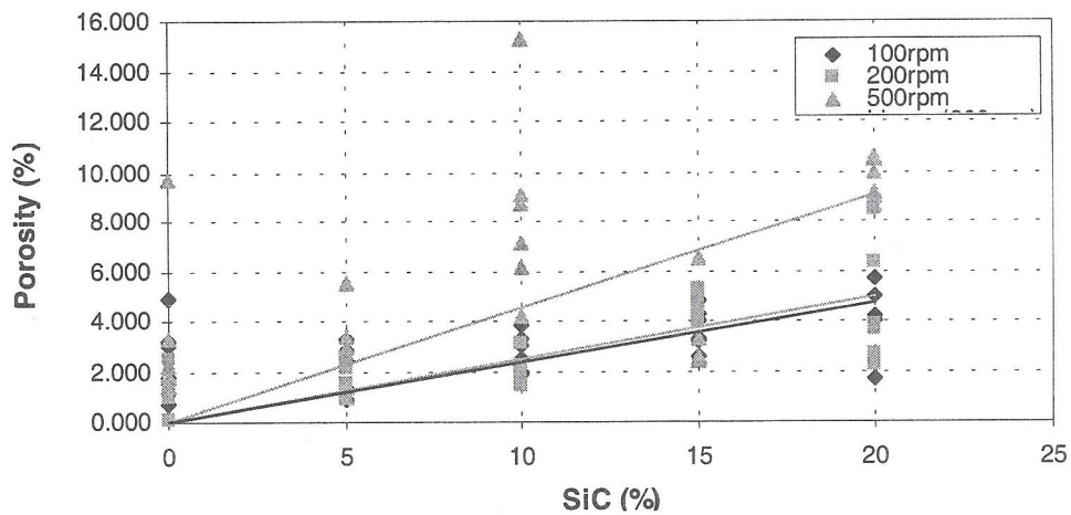
Figure 6 Porosity content of three different stirring speeds
