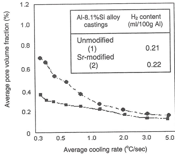
Figure 2 Average pore volume fraction as a function of average cooling rate for Al-8.1 wt % Si alloy cast [8]
