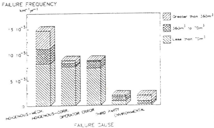
Fig. 7 Spill Volume Frequency By Failure Causes For European Crude Oil Pipeline \geq 16 in Diameter – CONCAWE Data [2]
