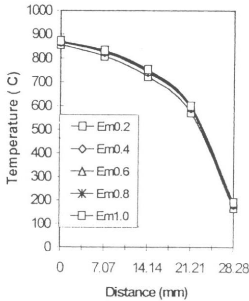
Fig. 10 Temperature Distribution Along Path C for Various Emissivities
