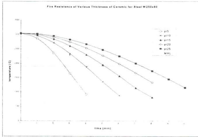
Fig. 4 Fire Resistance of Column for Different Insulation Thickness
