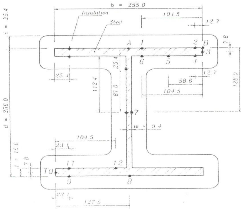
Fig. 1 Cross Section of Column
