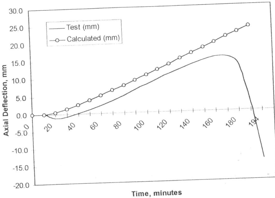
Fig. 11 Test and Calculated Values for Axial Deformation of Column FS5
