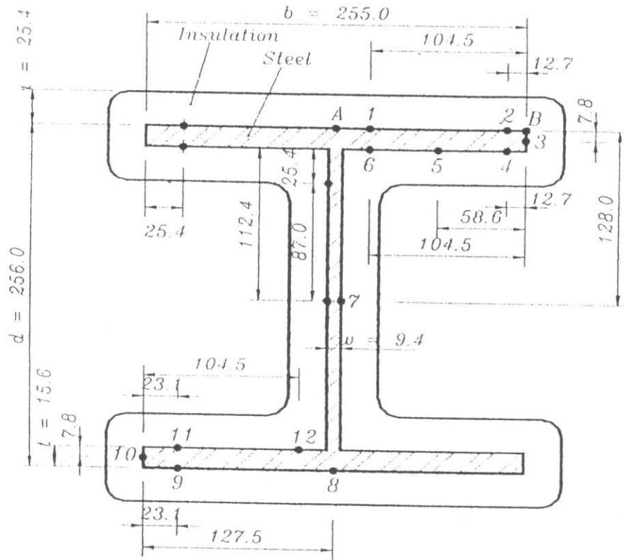
Fig. 1 W250-80 Steel Section with 1 Inch Ceramic
