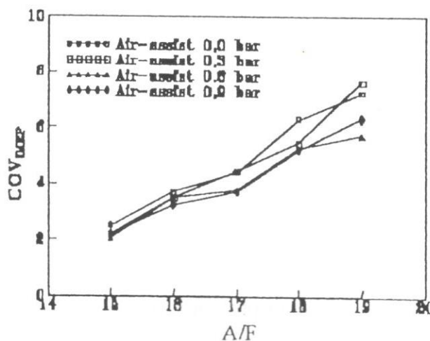
Fig. 10 Effect of Assist Air on COV imep
