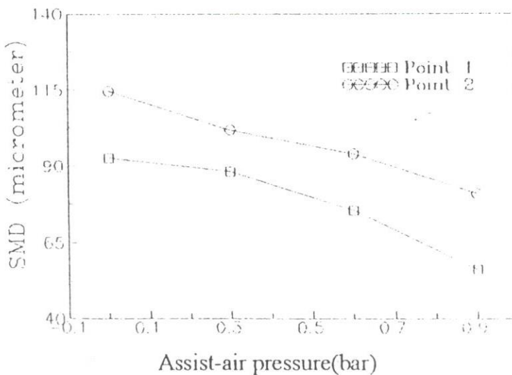
Fig. 8 Effect of Measuring Point on the SMD
