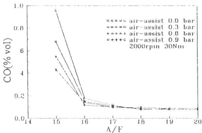
Fig. 12 Effect of Assist Air on CO Concentration
