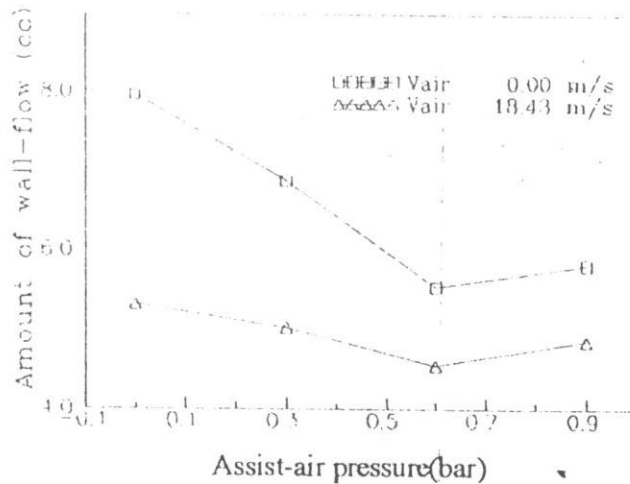
Fig. 9 Total Amount Of Wall-Flow
