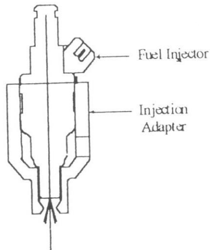
Fig. 1 Air-Assist Injection Adapter
