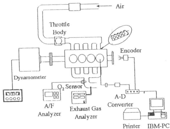
Fig. 5 Schematic Diagram of Test Engine
