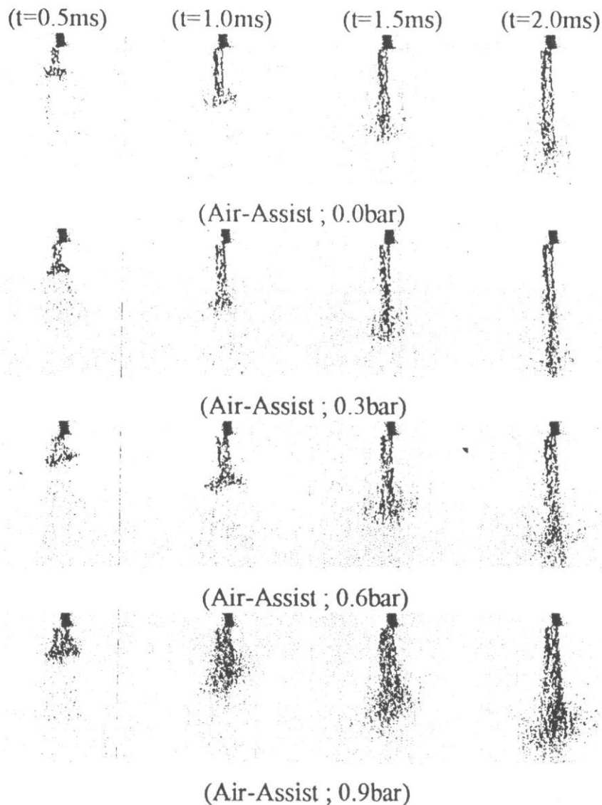
Fig. 6 Images Of Fuel Spray From Nozzle
