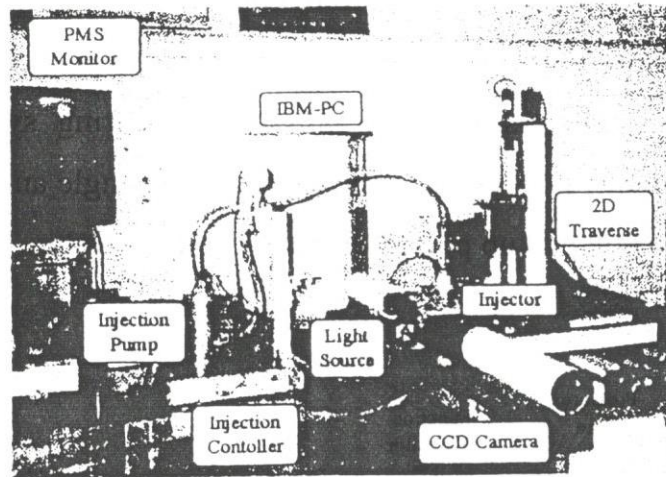
Fig. 2 Spray Particle Motion Analysis System
