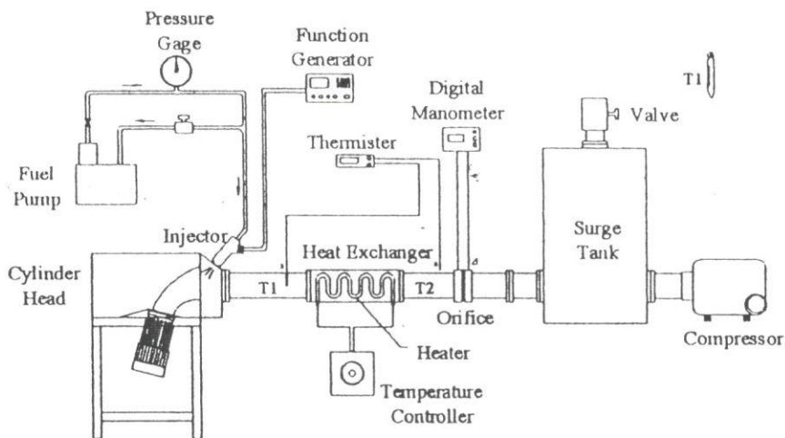
Fig. 4 Schematic Diagram Of Steady Flow Test Rig
