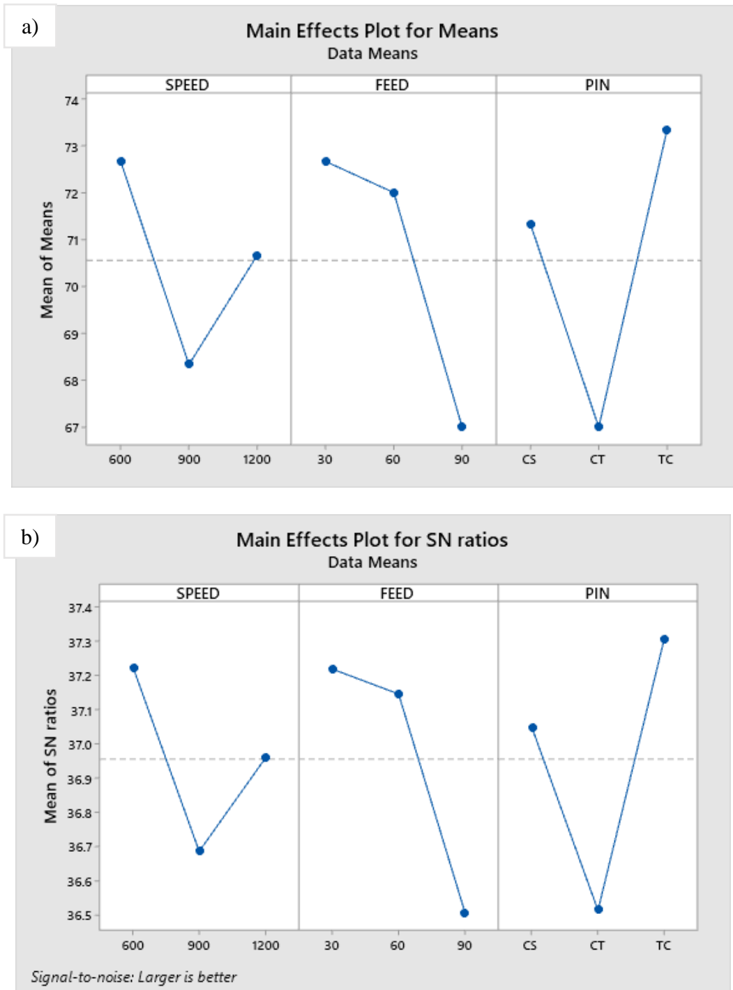
Figure 8: Main effect of welding parameters on hardness
