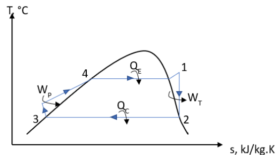
Figure 2: T-s diagram
